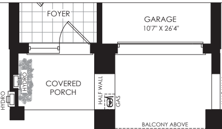
PARTIAL GROUND FLOOR PLAN ELEV. 'F'
