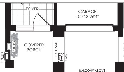
PARTIAL GROUND FLOOR PLAN ELEV. 'G'
