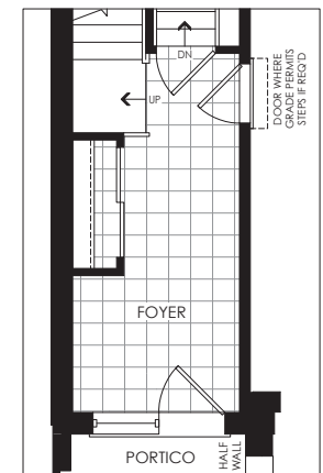
PARTIAL GROUND FLOOR PLAN FOR FLEX THIRD FLOOR PLAN WITH LAUNDRY
